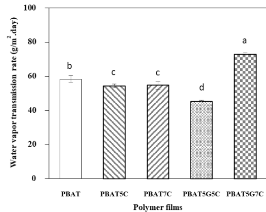
Figure 5 Water vapor transmission rate of PBAT, PBAT/CaCO 3 , and PBAT/Glycerol/CaCO 3 films.
